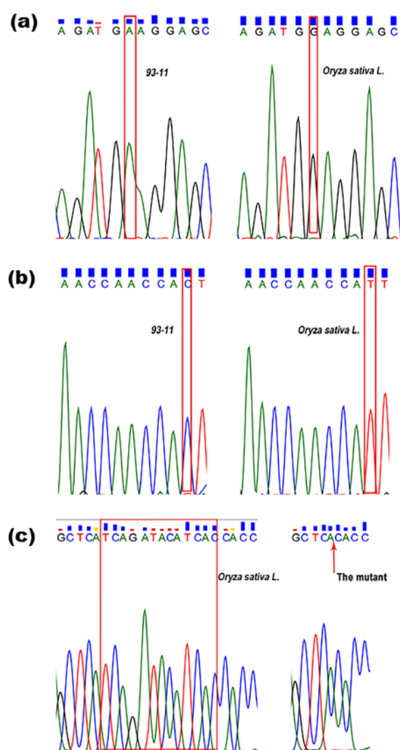
Supplemental Figure S1. Sanger sequencing of PCR amplification product reveals base mutations in different varieties of rice.
