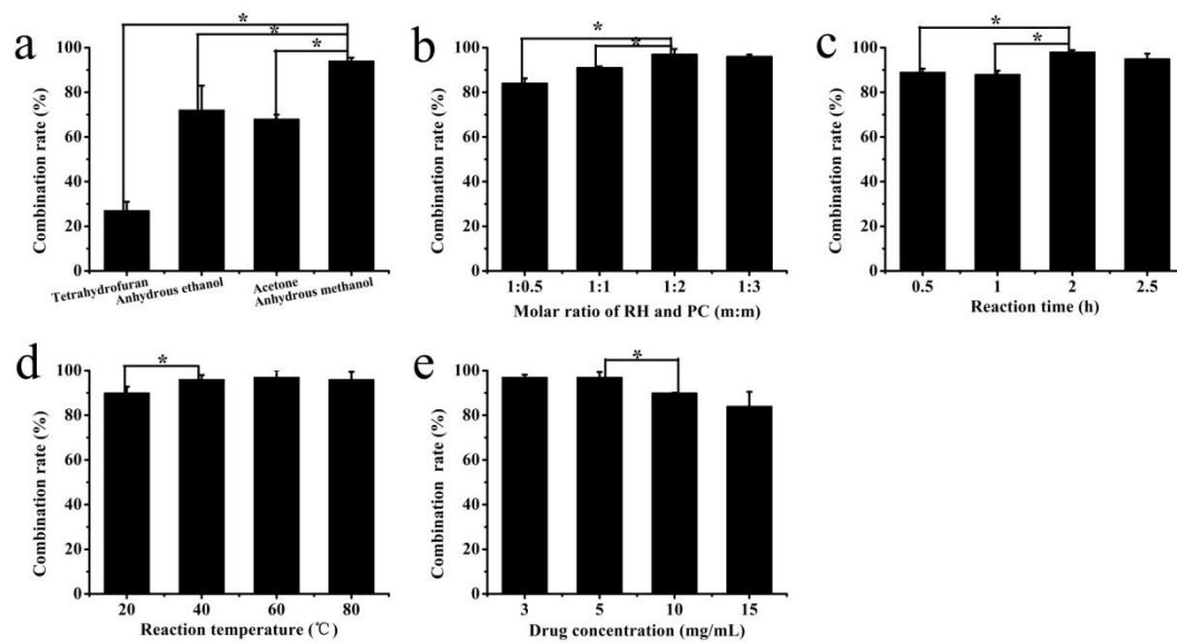
Figure S1 Combination rate of RHPC at different a types of solvent b RH-to-PC molar ratios, c reaction time, d reaction temperature, e RH concentration.
