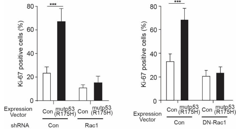
Supplementary Figure 1. The quantification of Ki-67 IHC staining in xenograft tumors formed by H1299-Con and H1299-R175H cells with or without knockdown of Rac1 by shRNA vectors (left panel), and with or without ectopic DN-Rac1 expression (right panel) . Data are presented as mean \pm SD. ***: p < 0.001 ; Student's t -test.
